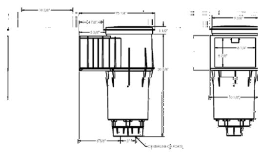
ADMIRAL S20 SKIMMER FOR CONCRETE
